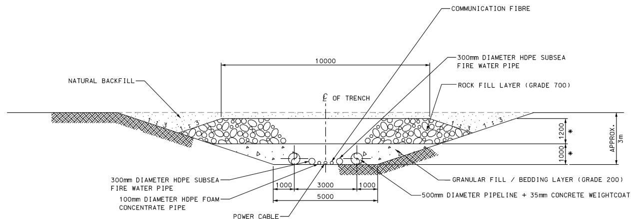
(A) CONCEPT SECTION THROUGH PIPELINE TRENCH BETWEEN JETTY AND PAFF
