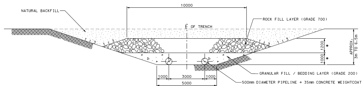
(B) CONCEPT SECTION THROUGH PIPELINE TRENCH BETWEEN PAFF AND SHA CHAU
